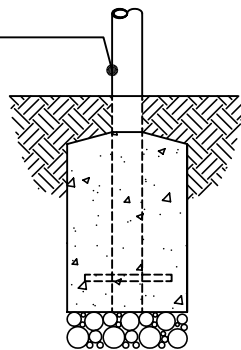
2153-6-ADA-E (DIRECT EMBEDMENT)
