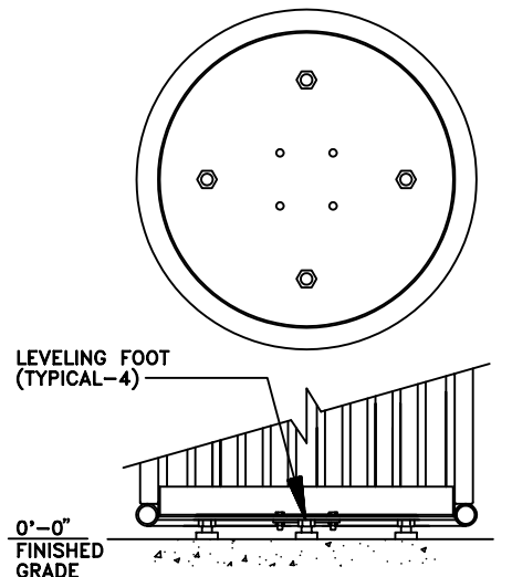
2772-AT-L (LEVELING MOUNT) SCALE: 3/4"=1'-0"
