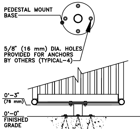
2772-AT-P (PEDESTAL MOUNT) SCALE: 3/4"=1'-0"
