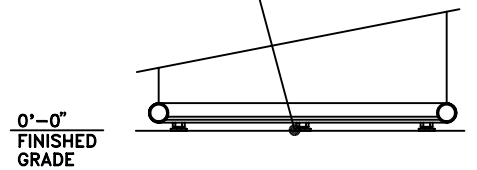
2814-FT-L (LEVELING MOUNT) SCALE: 3/4"=1'-0"
