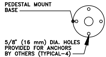
2814-FT-E (EMBEDMENT) SCALE: 3/4"=1'-0"
