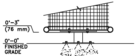
2891-FT-P (PEDESTAL MOUNT) SCALE: 3/4"=1'-0"
