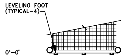
2891-FT-L (LEVELING MOUNT) SCALE: 3/4"=1'-0"
