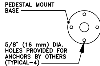
2891-FT-E (EMBEDMENT) SCALE: 3/4"=1'-0"
