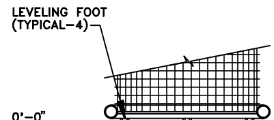
2891-HT-L (LEVELING MOUNT) SCALE: 3/4"=1'-0"
