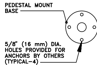
2891-HT-E (EMBEDMENT) SCALE: 3/4"=1'-0"
