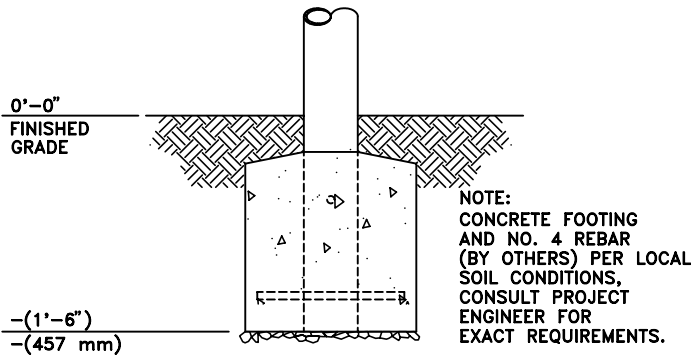
2912-0030-E (DIRECT EMBEDMENT)
