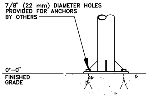
2912-0030-P (PEDESTAL MOUNT)
