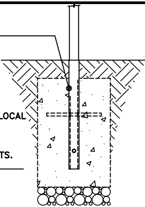
2921-20-E (DIRECT EMBEDMENT)
