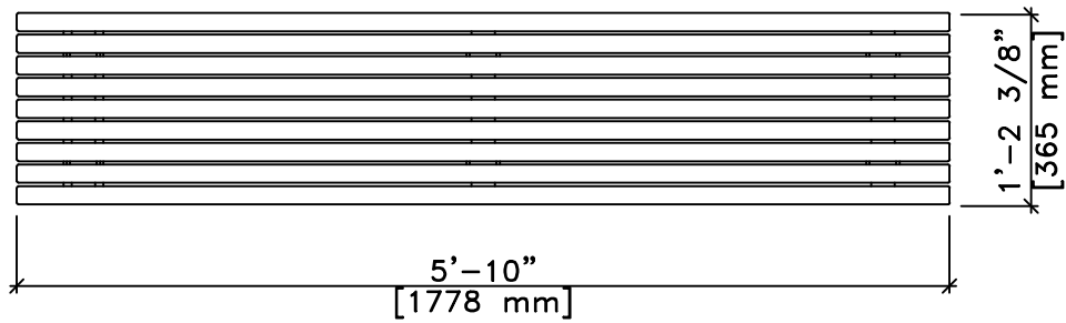
TOP VIEW
