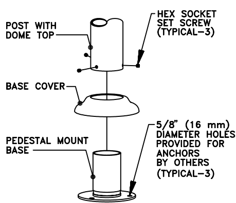
2190-P (PEDESTAL MOUNTING)
