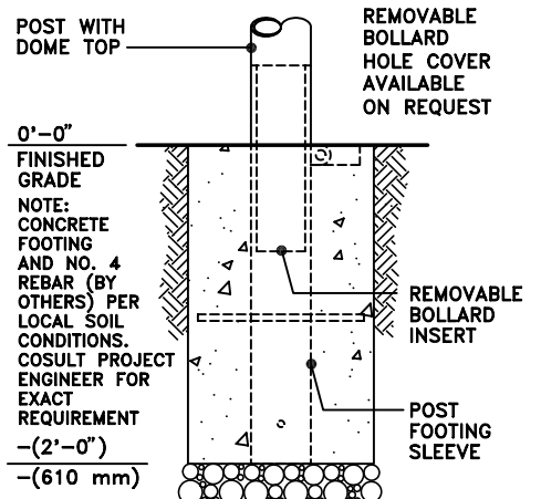
2190-R (REMOVABLE MOUNTING)
