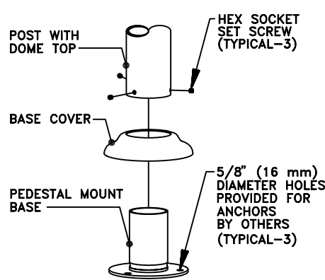
2197-P (PEDESTAL MOUNTING)
