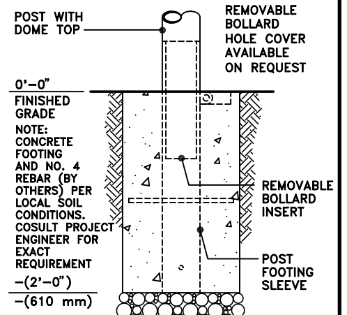
2197-R (REMOVABLE MOUNTING)
