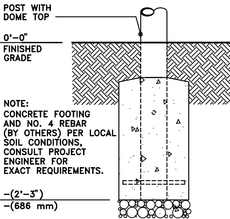
2197-E (EMBEDMENT MOUNTING)
