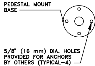
2811-FT-E (EMBEDMENT) SCALE: 3/4"=1'-0"
