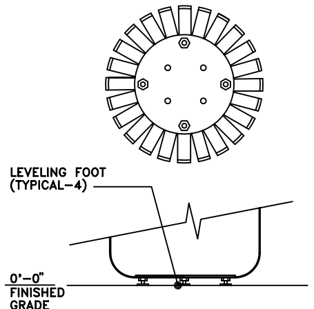
2811-FT-L (LEVELING MOUNT) SCALE: 3/4"=1'-0"
