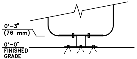
2811-FT-P (PEDESTAL MOUNT) SCALE: 3/4"=1'-0"
