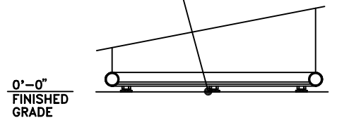
2814-OT-L (LEVELING MOUNT) SCALE: 3/4"=1'-0"
