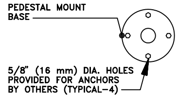
2814-OT-E (EMBEDMENT) SCALE: 3/4"=1'-0"
