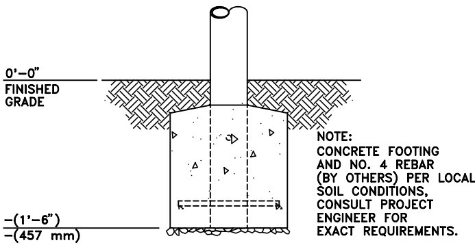
2902-0036-E (DIRECT EMBEDMENT)
