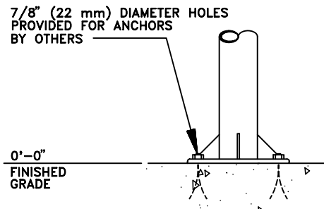
2902-0036-P (PEDESTAL MOUNT)
